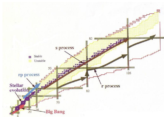
Figure 2. Path of nucleosynthesis at various sites. The decay properties and the capture reaction rates of unstable nuclei are essential for understanding these pathways and thus the elemental abundances
