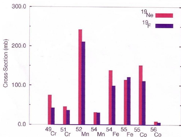
Figure 3. Comparison of fusion-evaporation production cross-sections of the reactions ^{19}\text{Ne} + ^{40}\text{Ca} and ^{19}\text{F} + ^{40}\text{Ca} at beam energies of 70 MeV
