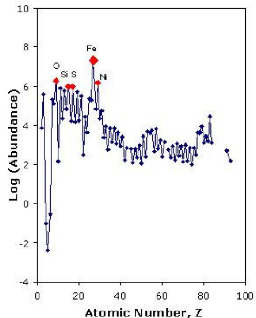
Figure 1. Relative abundance of the elements in the sun
