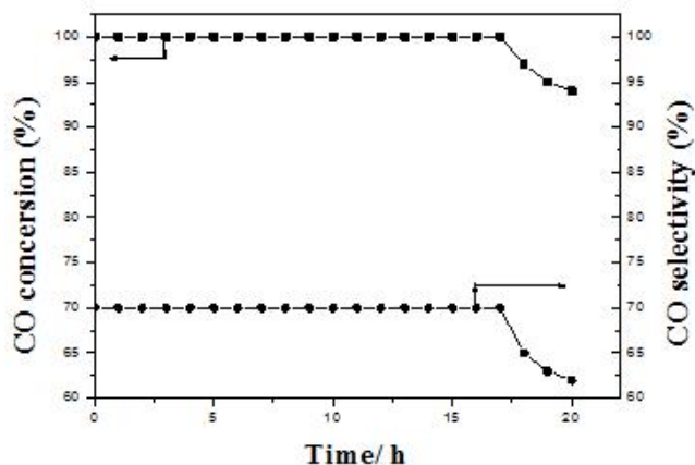
Fig. 9. Influence of moisture on the activity of catalyst 1.2% Rh/5A-400. (The feed gas consisted of 70% of H 2 , 2% of CO and 1.4% of O 2 , 10% of H 2 O and N 2 balance)
