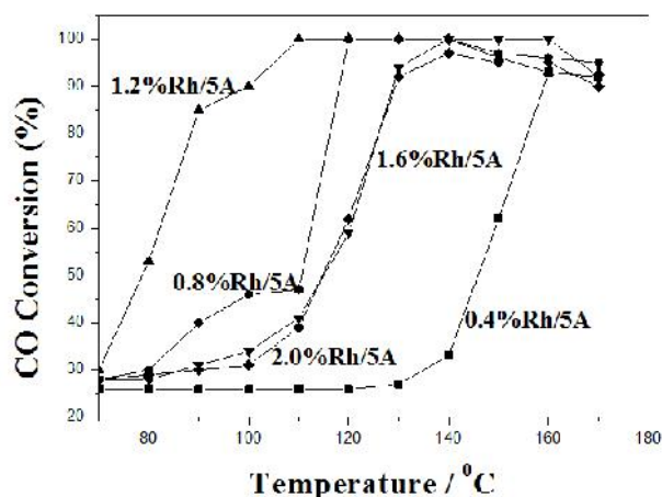
Fig. 4. Relation between reaction temperature and CO conversion for catalysts with different Rh-loading. (The total flow rate of the feed gas was 75 ml min -1 . The feed gas consisted of 70 % of H 2 , 2 % of CO and 1.4% of O 2 in N 2 balance)
