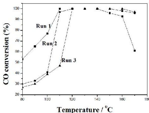
Fig. 8. Influence of moisture on the activity of catalyst 1.2% Rh/5A-400. (The feed gas consisted of 70% of H 2 , 2% of CO and 1.4% of O 2 , 10% of H 2 O and N 2 balance)
