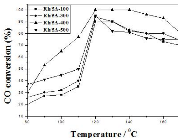
Fig. 6. Relation between reaction temperature and CO conversion for catalysts calcined at different temperature. (The total flow rate of the feed gas was 75 ml • min -1 . The feed gas consisted of 70 % of H 2 , 2% of CO and 1.4% of O 2 in N 2 balance)
