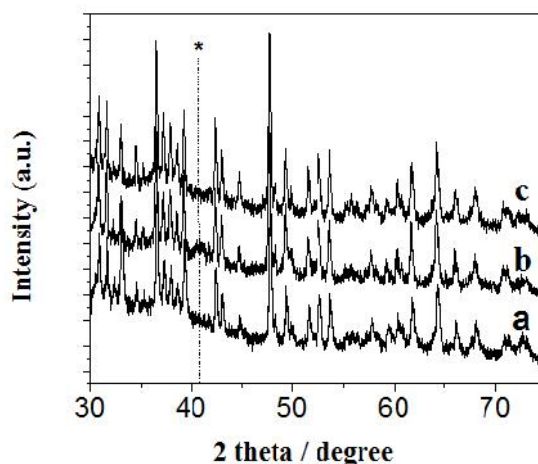
Fig. 1. XRD patterns of the catalysts calcined at different temperature (a) Rh/5A-200; (b) Rh/5A-400; (c) Rh/5A-500;
