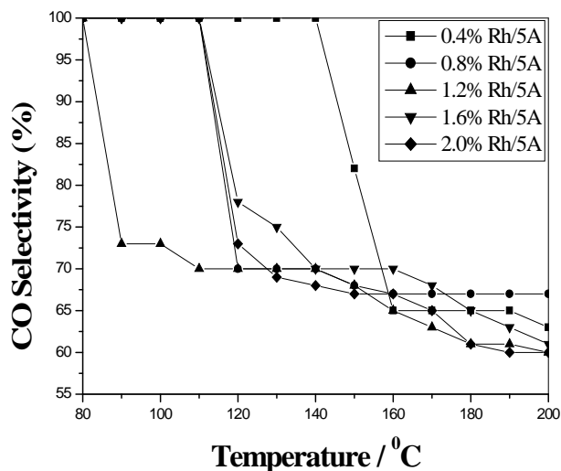
Fig. 5. Relation between reaction temperature and CO selectivity for catalysts with different Rh-loading. (The total flow rate of the feed gas was 75 ml • min -1 . The feed gas consisted of 70% of H 2 , 2% of CO and 1.4% of O 2 in N 2 balance)
