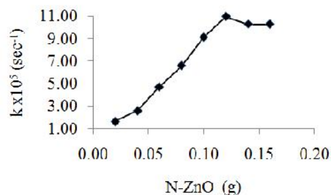
Fig. 5. Effect of amount of N-Doped ZnO
