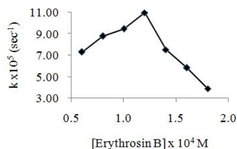
Fig. 4. Effect of Erythrosin B concentration
