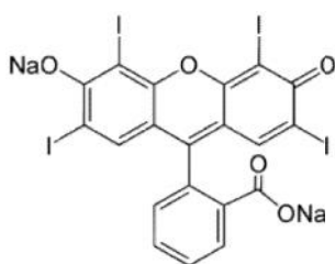
Fig. 1. Structure of Erythrosin B
