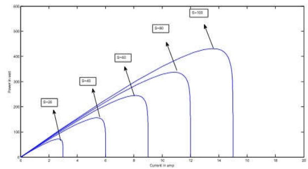
Figure 4.4. Power vs Current graph
