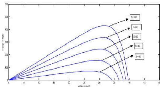
Figure 4.3: Power vs Voltage graph
