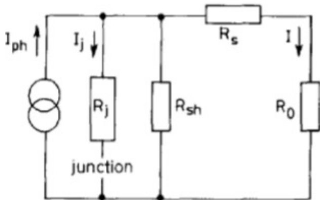
Figure 4.2. P-V Cell equivalent Circuit
