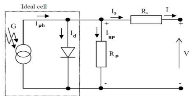
Figure 4.1. Electrical Equivalent Model of a Photovoltaic Cell
