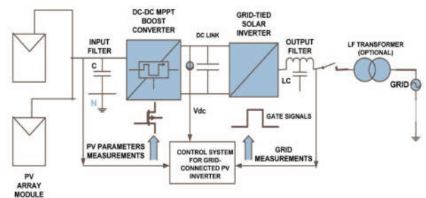
Figure 3.5. Systemic Scheme of rooftop SPV at DTU Campus
