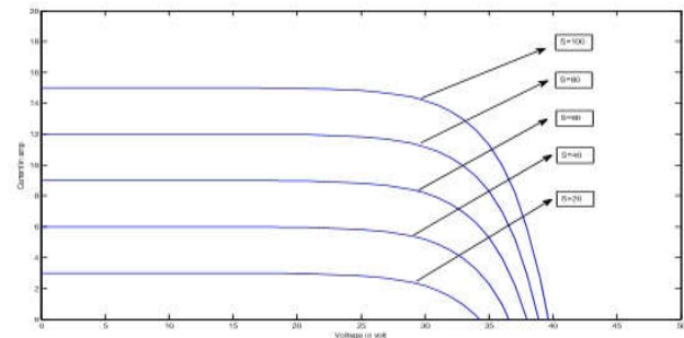
Figure 4.5. Current vs Voltage graph
